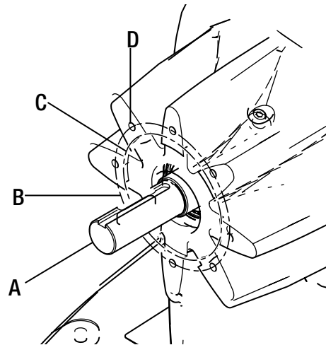
Motor mounting dimensions for EP3 & EP4 Pumps
